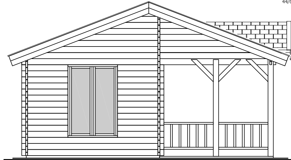
zyaanzicht (1) side view (1)
